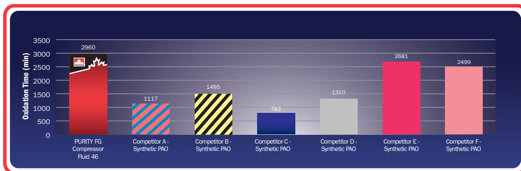
Resistance to Oxidation Rotating Pressure Vessel Oxidation Test, ASTM D2272
