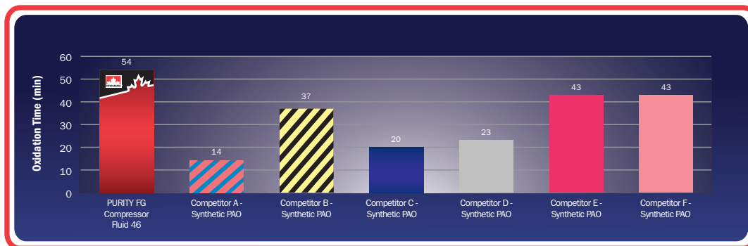
Resistance to Oxidation Pressure Differential Scanning Calorimetry, 200°C (392°F)
